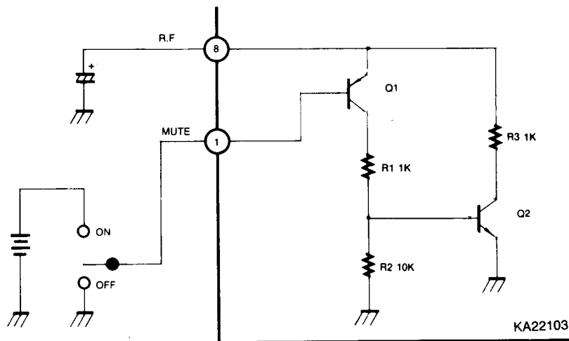
Fig. 7 MUTE Circuit
